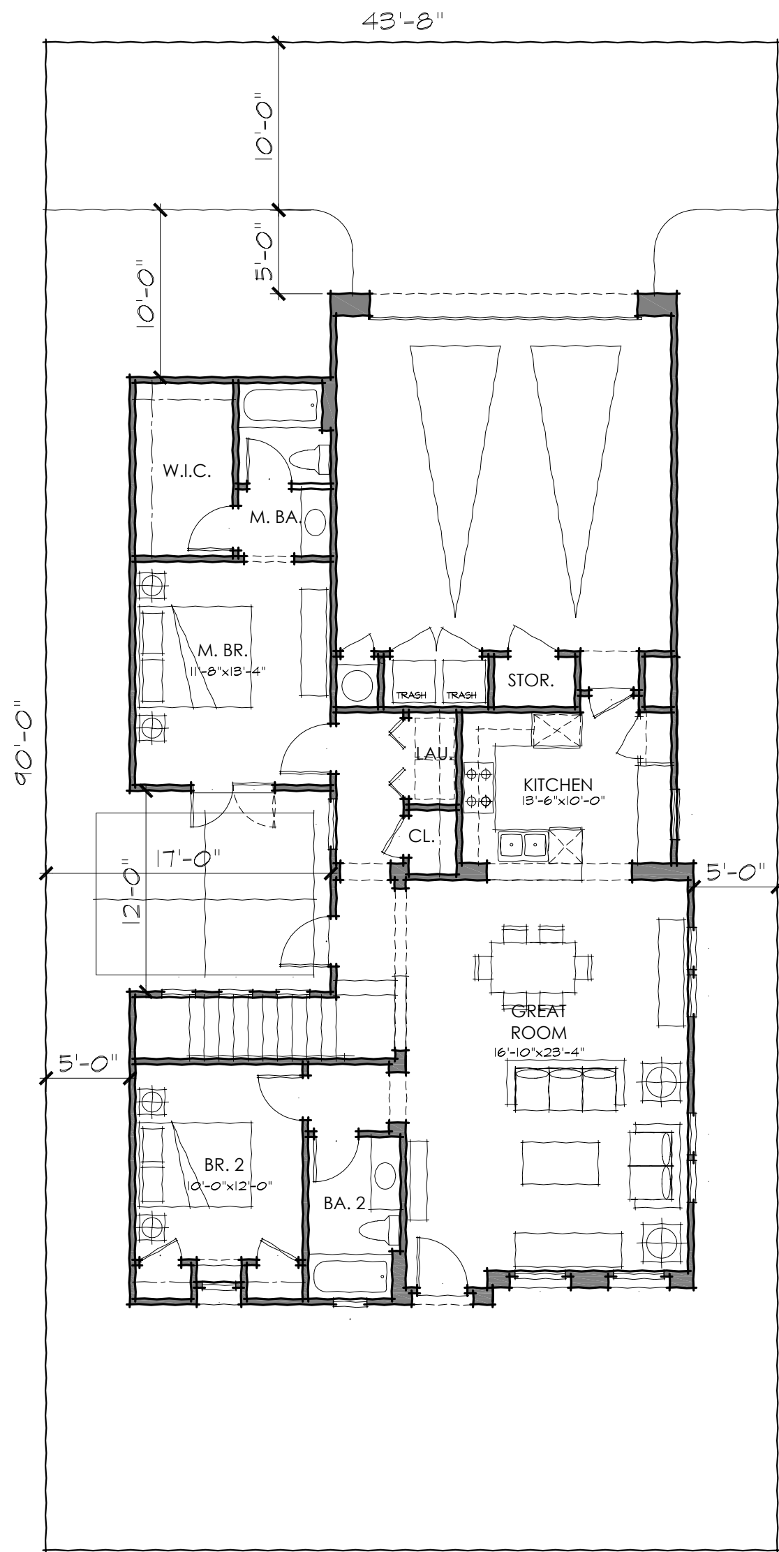
FIRST FLOOR
